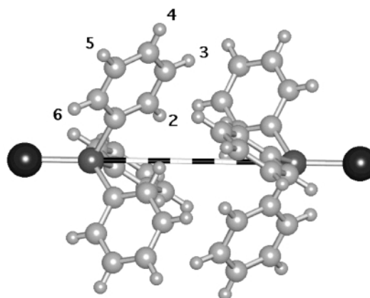
Fig. 1 A typical 6PE, showing the convention for numbering positions on the phenyl rings. Positions 2 and 3 correspond to o , m positions between pairs of P atoms in the interaction domain , while 6 and 5 represent o , m substitution away from the interaction domain. The 4-, 5- and 6-positions do not interfere with the 6PE. In this and all subsequent figures, black and white rods link the P atoms involved in the embrace.
