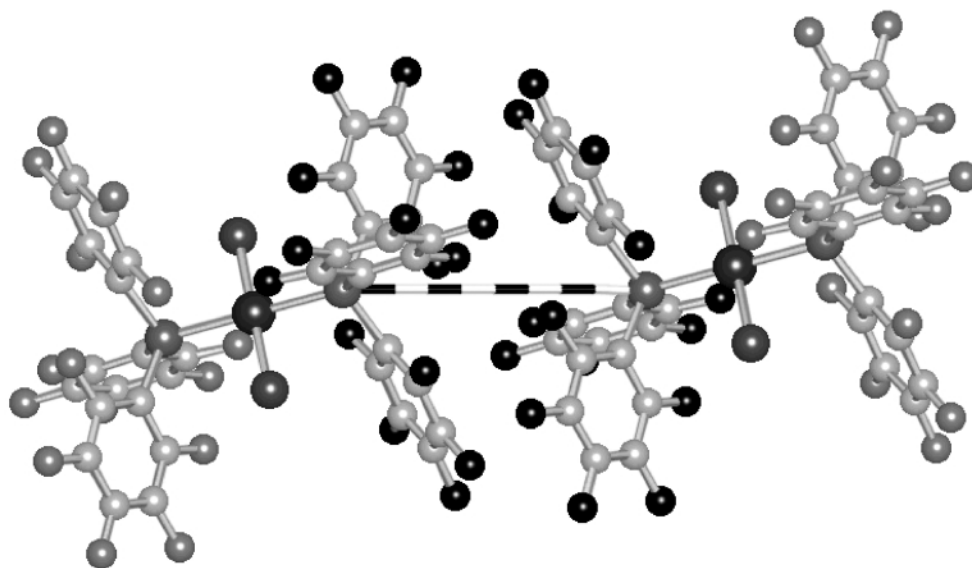
Fig. 7 The 6PE formed by the pentasubstituted compound [(\text{C}_6\text{F}_5)_3\text{P}]_2\text{Cl}_2\text{Pt} [VUBRIT]. The F atoms of the 6PE have been highlighted black. The symmetrical nature of the molecule leads to formation of chains of embraces.
